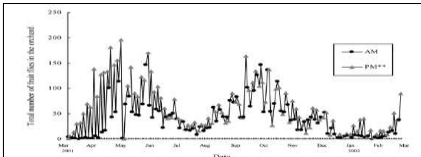
Fig. 3. Daily population changes of Bactrocera dorsalis in a guava orchard at Taiwan Agricultural Research Institute, Wufeng, Taichung, Taiwan. Captures were conducted twice a day at 9:00 am and 3:00 pm, and twice a week. Double asterisks indicate a significant difference between number of flies at different times at p < 0.01 (Student t test; SPSS 10.0 for windows 1999).
